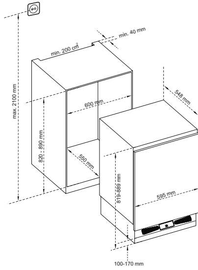
*820-828 for metal top cover
