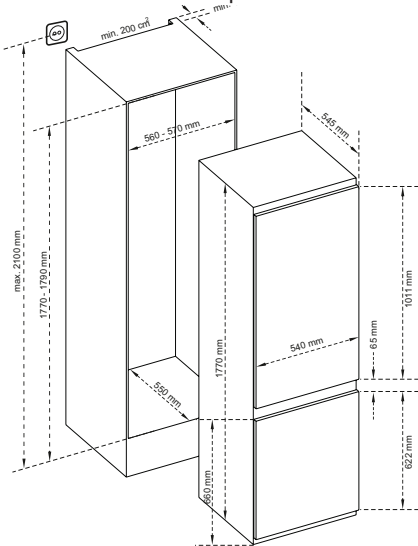
*1770-1778 for metal top cover
