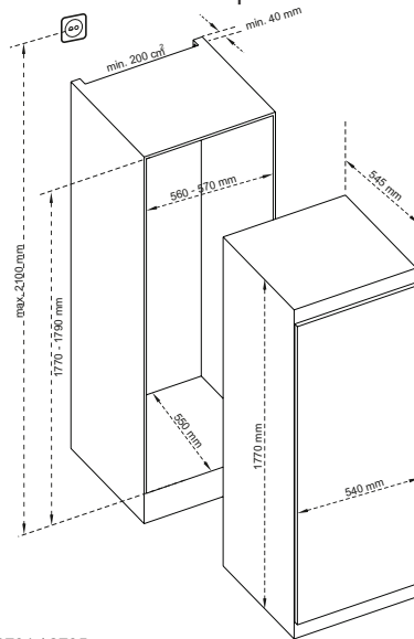
*1770-1778 for metal top cover
