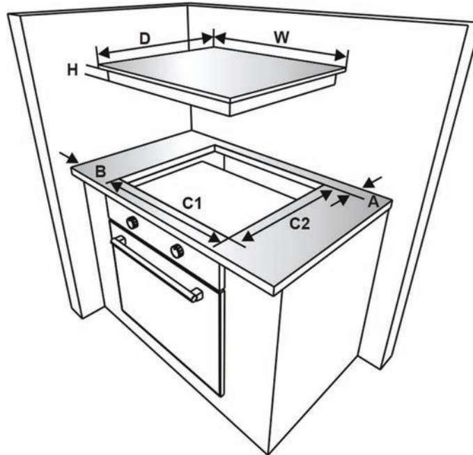
Installation dimensions for hob
