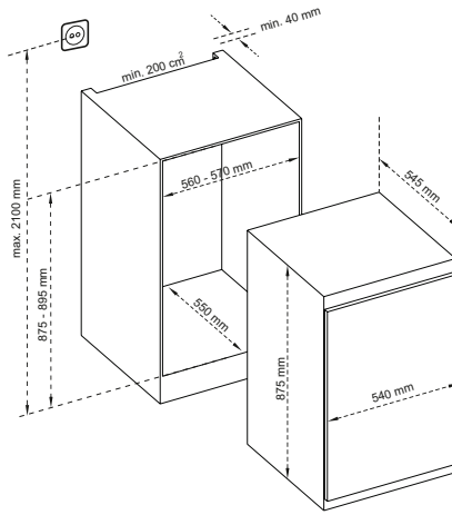
*875-883 for metal top cover
